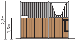
1-leaf door with V-opening in the battens Fixed part with upper vertical battens and dormer window for feeding
