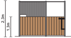
1-leaf door without battens Fixed part with upper vertical battens and dormer window for feeding
