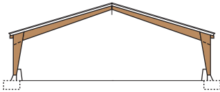
Portal trusses, 3 articulations
