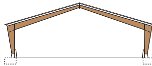
Portal trusses, 3 articulations Inverted pillars
